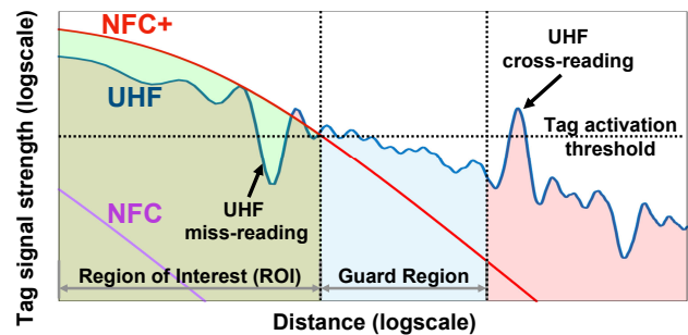
Figure 1: The propagation characteristics of the RF signal make UHF RFID unable to avoid miss-reading and cross-reading. In contrast, NFC+ leverages magnetic field to avoid miss-reading and cross-reading. Its operational range is significantly larger than NFC, which makes it suitable for logistics network applications.
