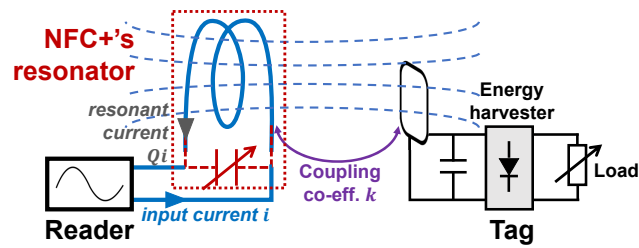
Figure 2: NFC reader-tag setup and close-loop magnetic coupling when tag is close to the reader. NFC+ leverages an additional high-Q resonator (simplified as the paralleled shunt capacitor and the coil inductor) which builds on top of NFC to boost the reading range.
