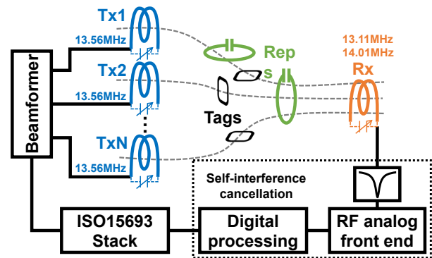
Figure 3: NFC+'s system overview
