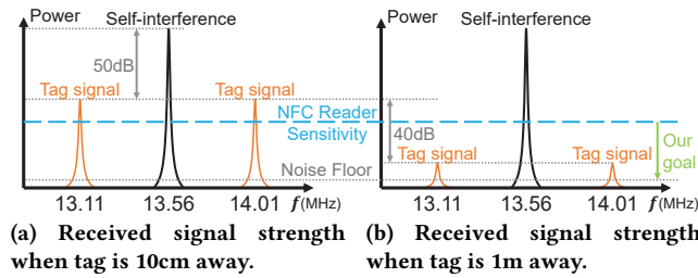
Figure 6: Self-interference experienced by a reader when a tag is placed at different distances from the reader.
