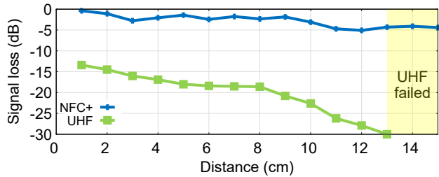
Figure 19: Signal degradation when tags are immersed in water. NFC+'s signal does not degrade a lot over distance while UHF RFID signal degrades significantly.
