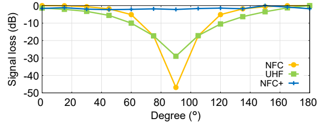
Figure 16: Performance of NFC+, state-of-the-art NFC, and UHF RFID with different tag orientations.
