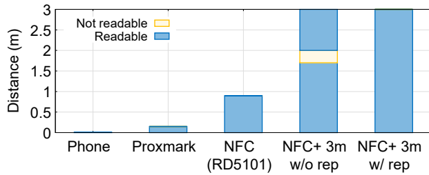
Figure 14: Comparative maximum operational distance.
