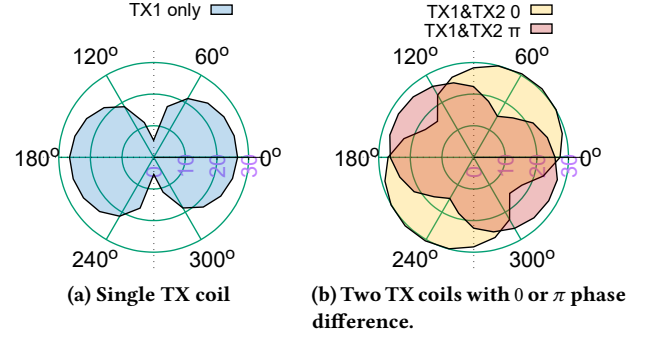
Figure 10: Beam patterns when using a single TX coil and two coils with magnetic beamforming.
