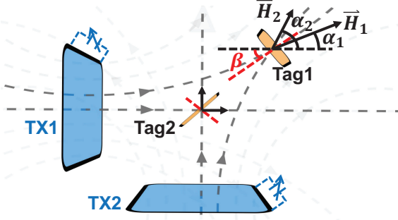
Figure 9: Two perpendicular TX coils setup and the vectors on the coordinate system.
