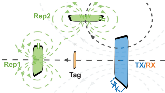
Figure 11: TX coil, mag-repeater placement and magnetic field line from TX coil and mag-repeater.
