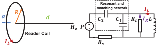
(a) Reader current loop model. (b) The equivalent circuit model.
