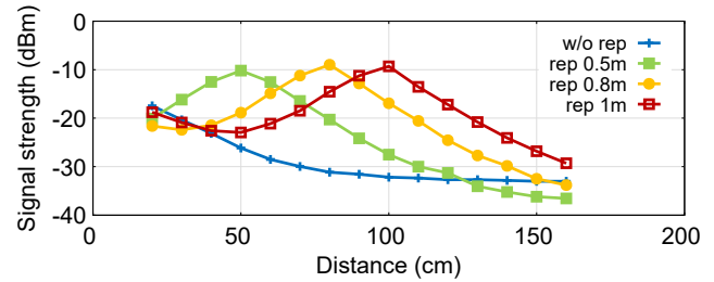
Figure 15: Mag-repeater helps improve the signal strength at long distances.
