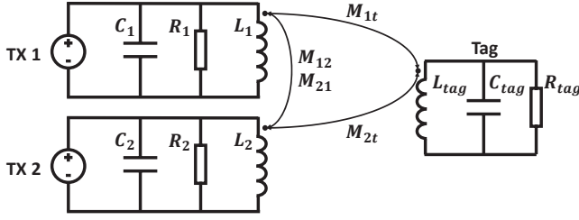
Figure 8: Circuit model of two TX coils setup.
